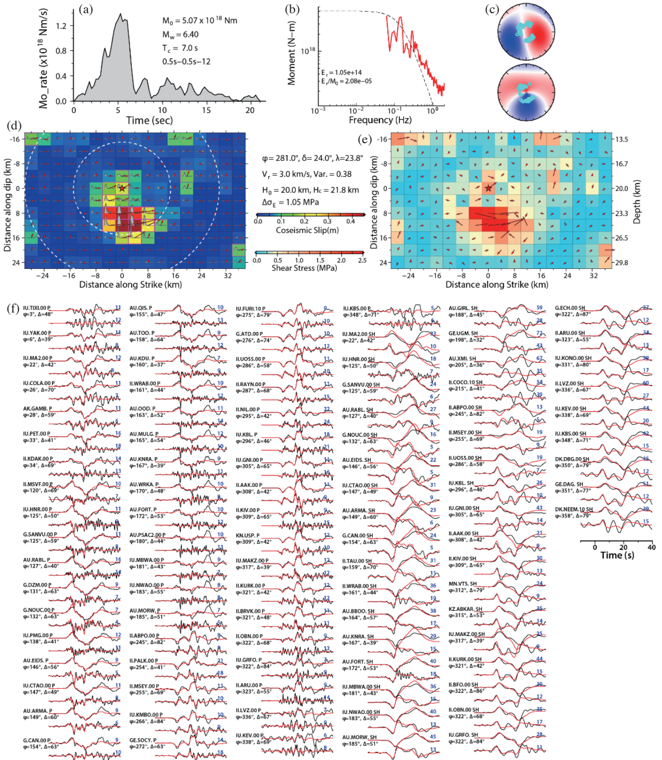
Fig. 4. Inversion of teleseismic body waves. (a) Moment-rate function and (b) moment-rate spectrum. (c) P and SH radiation patterns with the stations used for inversion. The mechanism is given by (slip/dip/rake = 281^\circ/24^\circ/24^\circ ), (d) Slip distribution, (e) distribution of stress drop, and (f) observed (black) and computed (red) teleseismic P and SH displacement and velocity waveforms. For each station, the first row shows the displacement and the second row shows the velocity. A rupture speed of 3 \text{ km s}^{-1} is assumed.
