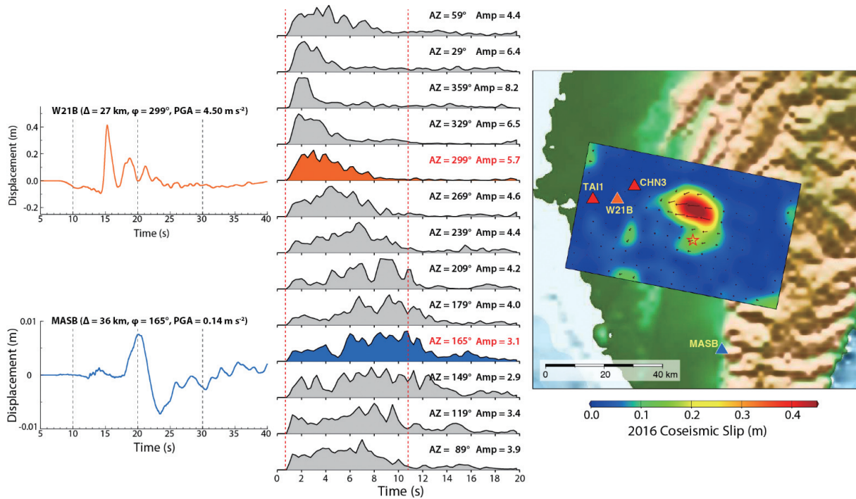
Fig. 11. The moment-rate functions (shaded pattern) viewed from various azimuths. The slip distribution is shown on the right. The stations W21B and MASB are located in the azimuth of 299° and 165°. The moment-rate functions viewed from the azimuth of W21B and MASB are shown in red and blue, respectively. The displacement record at the respective station is shown for comparison.
