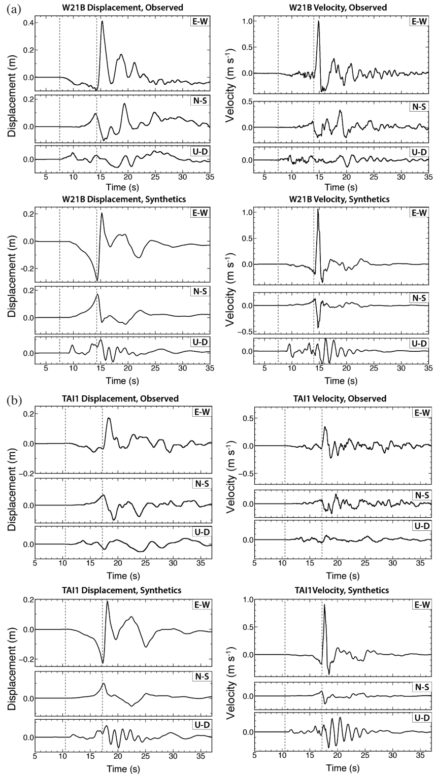
Fig. 12. Comparison of the observed (top) and synthetic (bottom) waveforms for the station (a) W21B, (b) TAI1, and (c) CHN3. Three-component displacement and velocity waveforms are shown. The “soft” crustal structure model is used.
