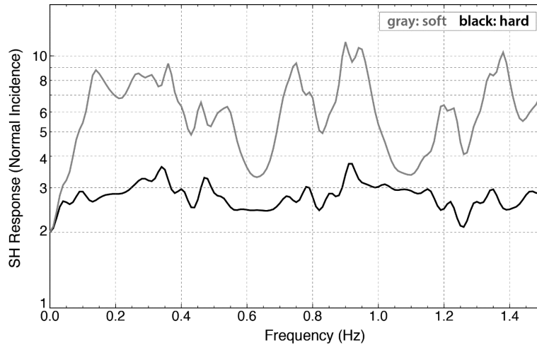
Fig. 10. Crustal response functions for a vertically incident SH waves for the “soft” (gray curve) and “hard” (black curve) crustal structure models.
