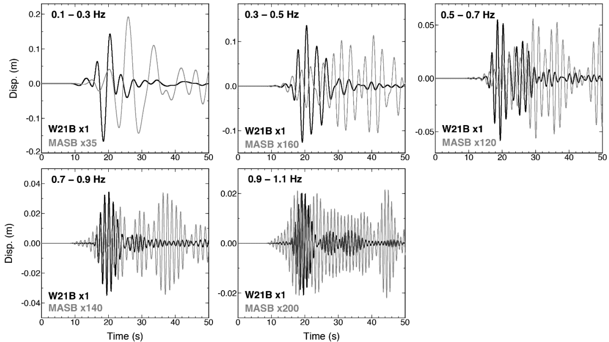
Fig. 6. Comparison of the amplitude at W21B (black) and at MASB (gray) at 5 frequency bands. For each frequency band the records are Butterworth band-pass filtered. For comparison, the MASB record is multiplied by a factor given at the lower left of each figure. Note that at the frequency band 0.3 - 0.5 Hz (2 - 3.3 s); the amplitude ratio is about 160.
