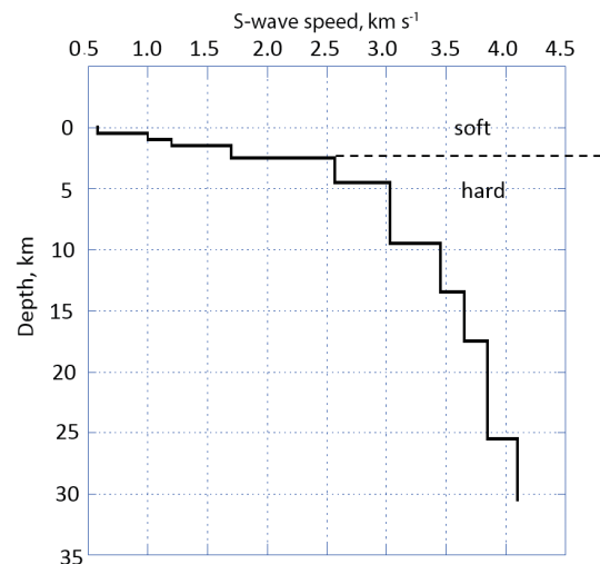
Fig. 8. S-wave vertical profile used for the “soft” structure model. The “hard” structure model is obtained by removing the top 5 layers above the depth indicated by a dashed line. (Color online only)
