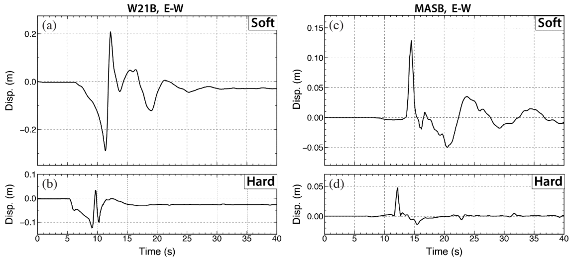
Fig. 9. Synthetic displacement waveforms computed for the stations W21B and MASB using the “soft” and “hard” structure models.
