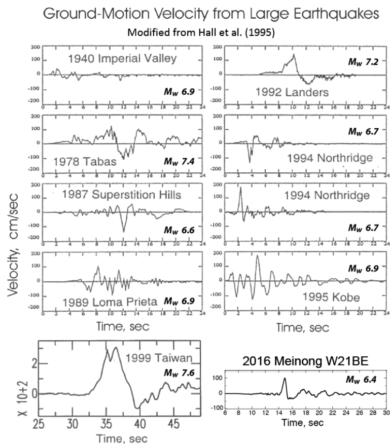
Fig. 2. Ground-motion velocity recorded at W21B (EW component) for the 2016 Meinong earthquake compared with the S-wave pulses of damaging large earthquakes in the past (modified from Hall et al. 1995). Note the similarity of the waveforms between the 1994 Northridge earthquake and the 2016 Meinong earthquake.
