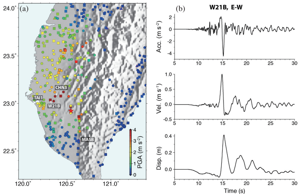
Fig. 1. (a) PGA distribution of the 2016 Meinong earthquake (circles: CWB stations; squares: Palert stations; triangles: BATS stations). The epicenter is indicated by a star, and the 4 stations discussed are indicated by their station names. (b) The EW component ground-motion acceleration, velocity and displacement recorded at a Palert station W21B. The ground-motion waveforms recorded at station MASB are shown in Figs. 5, 11, and 13.
