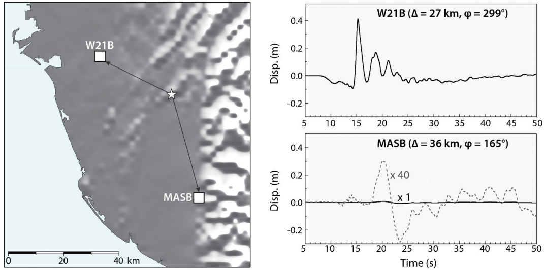
Fig. 5. Comparison of the EW component displacement waveforms at the stations W21B and MASB. On the plot for MASB, the black curve (marked as \times 1 ) is the plot with the same amplitude scale as that for W21B, and the gray curve ( \times 40 ) shows the displacement multiplied by 40, indicating that the trace amplitude at W21B is about 35 times larger than that at MASB. (Color online only)
