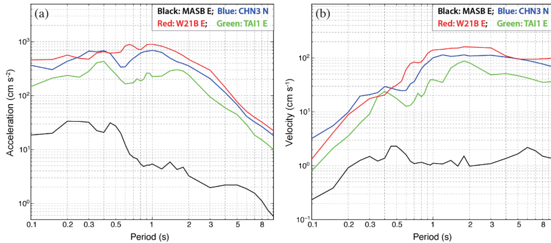
Fig. 7. Spectral acceleration (a) and spectral velocity (b) computed for the records at MASB (EW component), W21B (EW component), CHN3 (NS component), and TAI1 (EW component). Damping is 5%. (Color online only)
