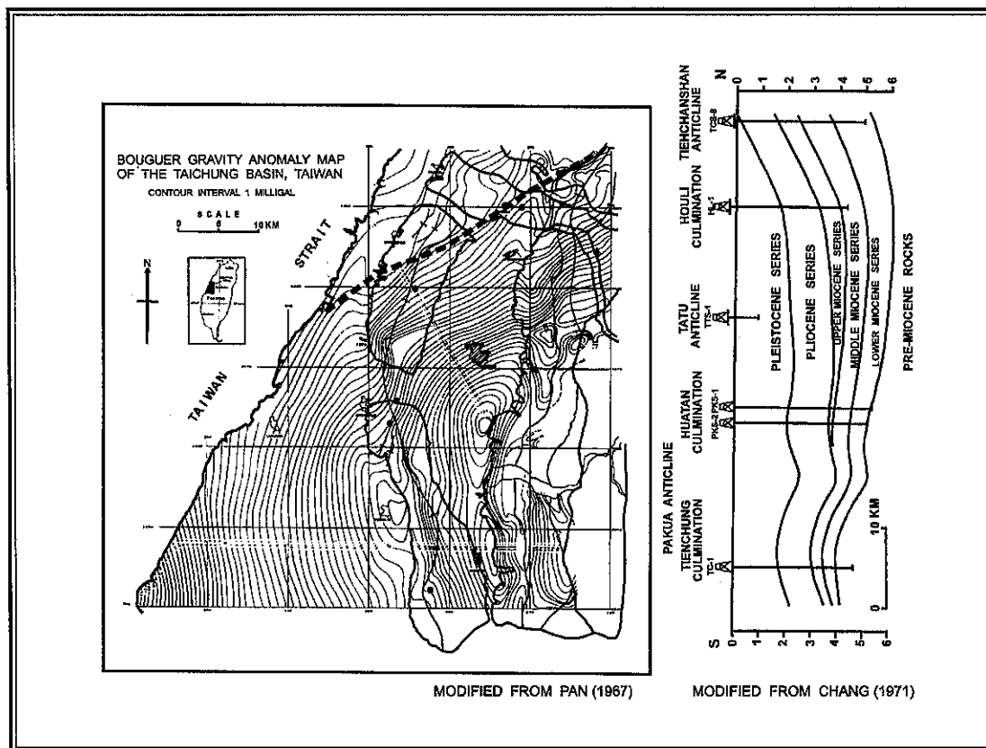
Fig. 3. The Bouguer gravity anomaly map and a NS profile in the central Taiwan region (adopted from Pan 1967 and Chang 1971). An abrupt change of contours occurs in the northwest. The dashed line trending NE-SW separates the high and low gravity gradient regions (i.e., the buried Tai-an fault). Two structural highs (the Tienchung and Huatan culminations) are identified to the south. The structure arises north of the Houli terrace, then enters the Tiehchanshan anticline region in the north.
