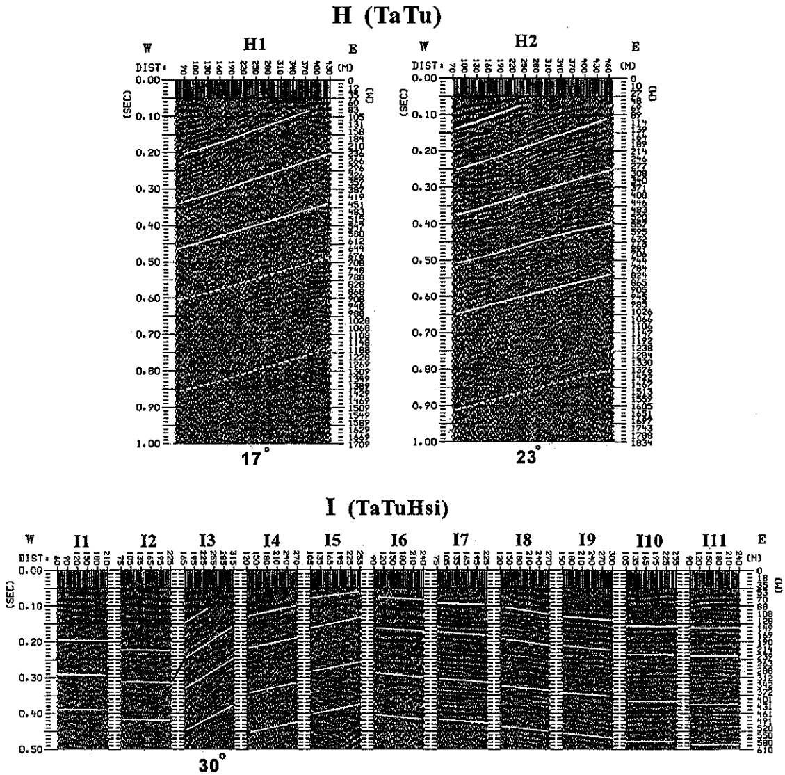
Fig. 12. Profile H (top) contains two sections (H1 and H2) located directly at the position of the suspected Changhua fault north of the Tatuhsi river. The bending of the layers is quite clear, with dip angles greater than 15 degrees. Profile I (bottom) is a consecutive section profile made along the southern bank of the Tatuhsi river. A fault-bend-fold structure sits in the middle, which has a step front with a dip angle of more than 25 degrees and an anticline at the back. This high angle indicates that the axis of Tatu-Pakua anticline may reach its climax at the position of the Tatuhsi river.
