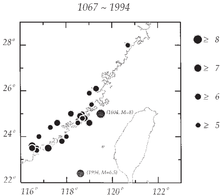
Fig. 1. Seismicity of major earthquakes of Quanzhou-Shantou and Taiwan Strait regions from 1067 to 1994 (Kuo and Ma, 1988). Two large earthquakes (1604 and 1994) are marked with their magnitude given.
