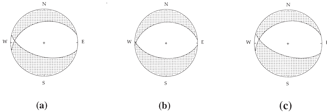
Fig. 7. The best double couple fault plane solutions of the 16 September 1994 Taiwan Strait earthquake determined by different groups. (a) Kao and Wu (1996), (b) Zheng et al. (1998) and (c) The Harvard solution (Dziwonski et al., 1995).
