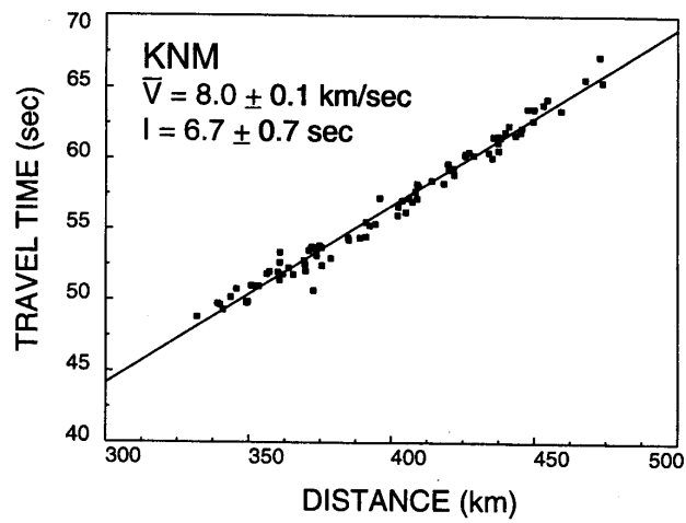
Fig. 5. Plot of source depth corrected travel times vs. distance for station KNM. \bar{V} and I represent the estimated Pn velocity and intercept time, respectively. The error range was estimated by one standard deviation of data and was the same as other figures in this study.
