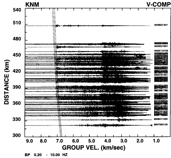
Fig. 4. Vertical seismograms recorded by station KNM as a function of group velocity to allow for a direct comparison of the traces. The vertical axis represents the source depth corrected epicenter distance. Amplitudes were normalized using individual amplitude maximum of trace. The solid lines represent travel time curves with P_n velocities of 8.1, 8.0 and 7.9 km/sec from left to right. More details are provided in the text.
