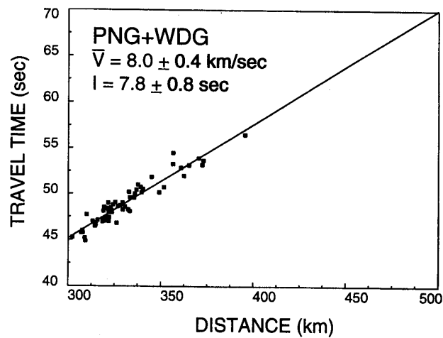
Fig. 6. Plots of source depth corrected travel times vs. distance for stations PNG and WDG. \bar{V} and I represent the estimated Pn velocity and intercept time, respectively.
