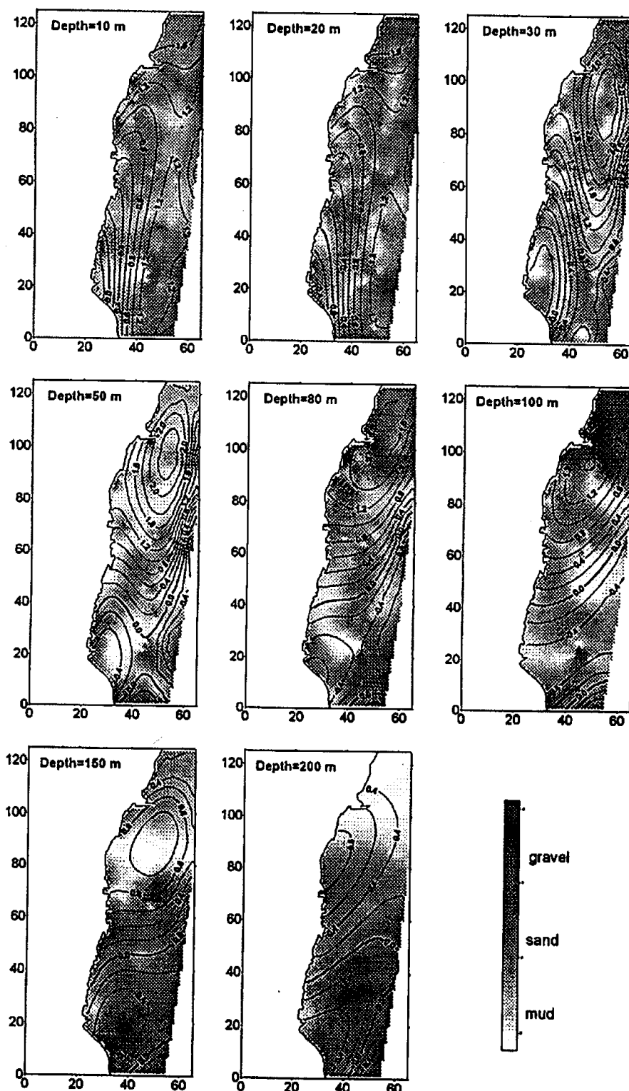
Fig. 9. Regional resistivity contour maps (in log 10 resistivity, ohm-m) at depths 10, 20, 30, 50, 80, 100, 150 and 200 m, respectively, are superimposed on lithofacies distributions which are displayed in shaded maps. The correlation between the locations of higher resistivity contours ( in the north ) and the regions of gravel or sand is noteworthy.
